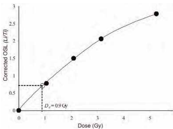
Figure 2. Dose-response curve of quartz extracted from sample PRF3-3 can be described by an exponential function for a dose range from 0 to 5 Gy. The equivalent dose is found from corrected natural OSL signal ( L_n/T_n ).
