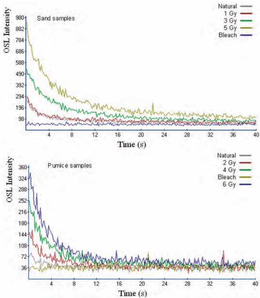
Figure 3. OSL decay curves of quartz from representative sandy and pumice samples. OSL signals were recorded from natural, bleached and irradiated aliquots; 1 Gy, 3 Gy and 5 Gy for sand samples and 2 Gy, 4 Gy and 6 Gy for pumice samples.
